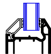
20mm Glazing
