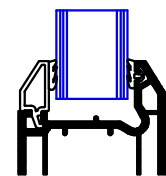
28mm Glazing
