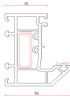
701501 56mm Outer Frame Steel U Channel 713185 Steel Box 713155 Steel Box 713187
