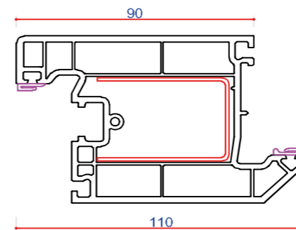
705510 (P10510) Door Sash - Open In Steel U Channel 713162 Punched Steel U 713163
