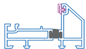
704345 (A00345) French Door Low Threshold
