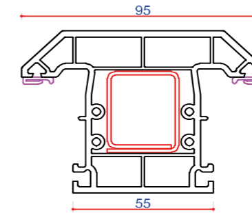
702504 (P10504) 95mm T Transom Steel Box 713174 Steel Box 713191 Steel Box 713157
