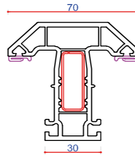
702503 (P10503) 70mm T Transom Steel Box 713187 Steel Box 713155 35 x 12.5 Ported Alu 715161
