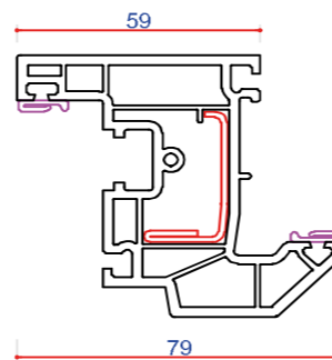
703509 (P10509) Tilt & Turn Sash Steel L Section 713161
