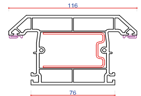
702505 (P10505) 116mm Midrail Steel U Channel 713166 35 x 58 Ported Alu 715163
