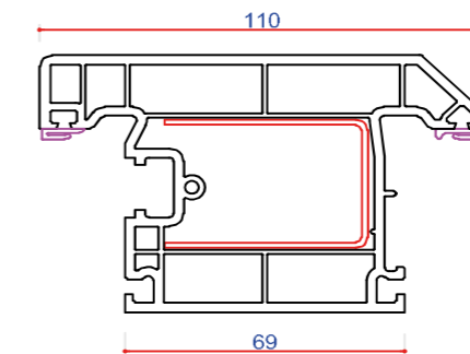
705511 (P10511) Door Sash - Open Out Steel U Channel 713162 Punched Steel U 713163
