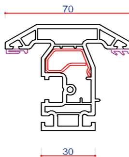
703514 (P10514) Internally Beaded Sash / Transom Steel P Section 713183 Steel P Section 713184
