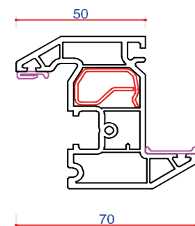
703507 (P10507) Externally Beaded Sash Steel P Section 713182
