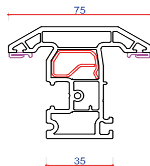
703508 (P10508) Internally Beaded Sash Steel P Section 713182
