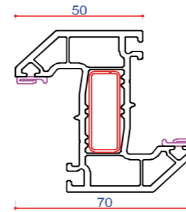
702506 (P10506) 70mm Z Transom Steel Box 713187 Steel Box 713155
