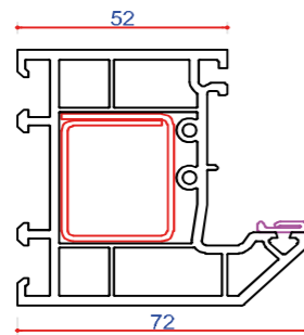
701502 (P10502) 72mm Outer Frame Steel Box 713174 Steel Box 713191 Steel U Channel 713186 Steel P Section 713157 Thermal Insert 709332
