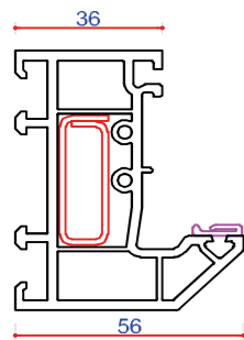
701501 (P10501) 56mm Outer Frame Steel Box 713155 Steel Box 713187 Steel U Channel 713185 Thermal Insert 709331
