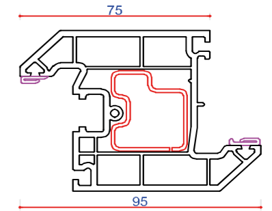
705515 (P10515) 95mm Z Transom Steel Box 713158
