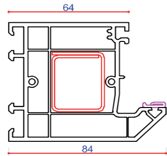
701203 84mm Outer Frame Steel Box 713174 Steel Box 713191 Steel U Channel 713186 Steel P Section 713157 Thermal Insert 709332
