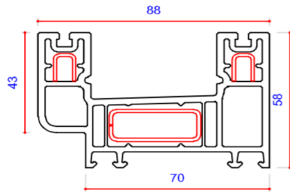
105178 58mm Outer Frame Steel U Channel 113018 Steel Box 713104
