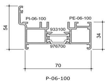
Rebated Threshold
